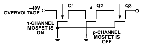
Figure 32. -40 V Overvoltage with Power Off
