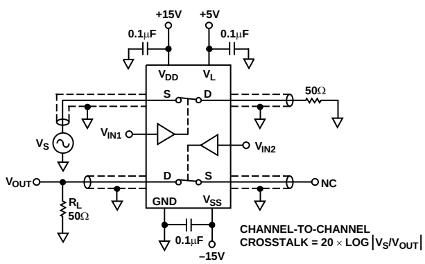
Figure 21. Channel-to-Channel Crosstalk
