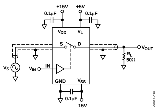
Figure 20. Off Isolation
