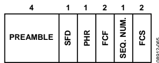
Figure 89. ACK Frame Format
