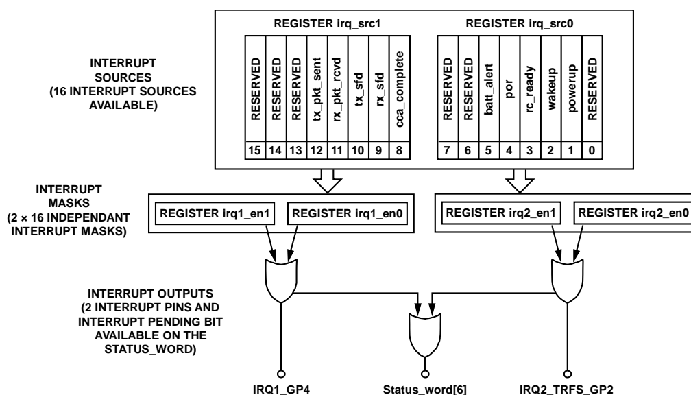
Figure 114. Interrupt Controller
