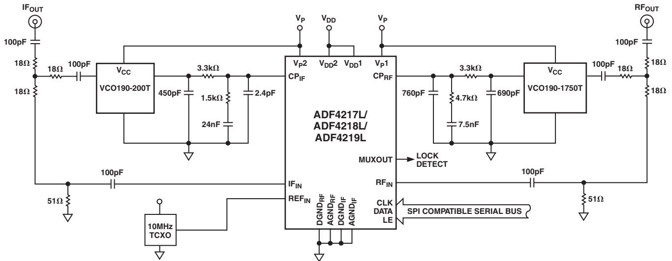
Figure 8. Local Oscillator Design for WCDMA System
