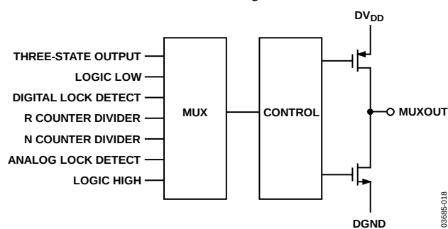
Figure 16. MUXOUT Schematic
