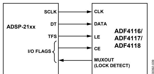
Figure 39. ADSP-21xx to ADF411x family Interface
