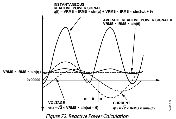
Figure 72. Reactive Power Calculation
