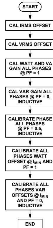
Figure 81. Calibration Using Line Accumulation
