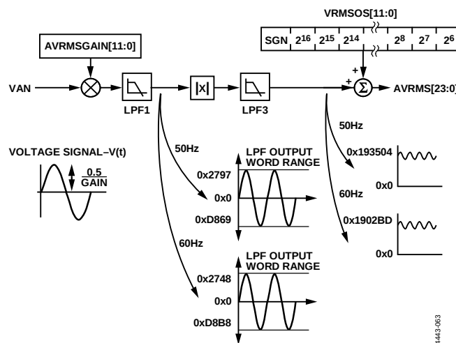
Figure 64. Voltage RMS Signal Processing
