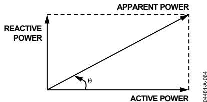
Figure 63. Power Triangle
