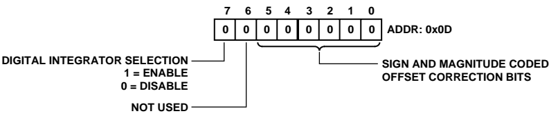
Figure 88. Channel 1 Offset Register
