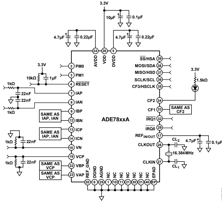
Figure 23. Test Circuit
