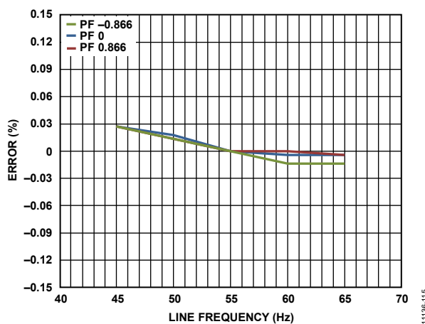
Figure 15. Total Reactive Energy Error as a Percentage of Reading (Gain = +1) vs. Line Frequency over Power Factor with Internal Reference and Integrator Off
