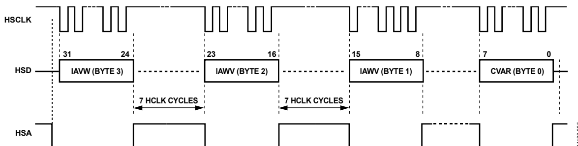
Figure 103. HSDC Communication for HSIZE = 1, HGAP = 1, HXFER[1:0] = 00, and HSAPOLE = 0
