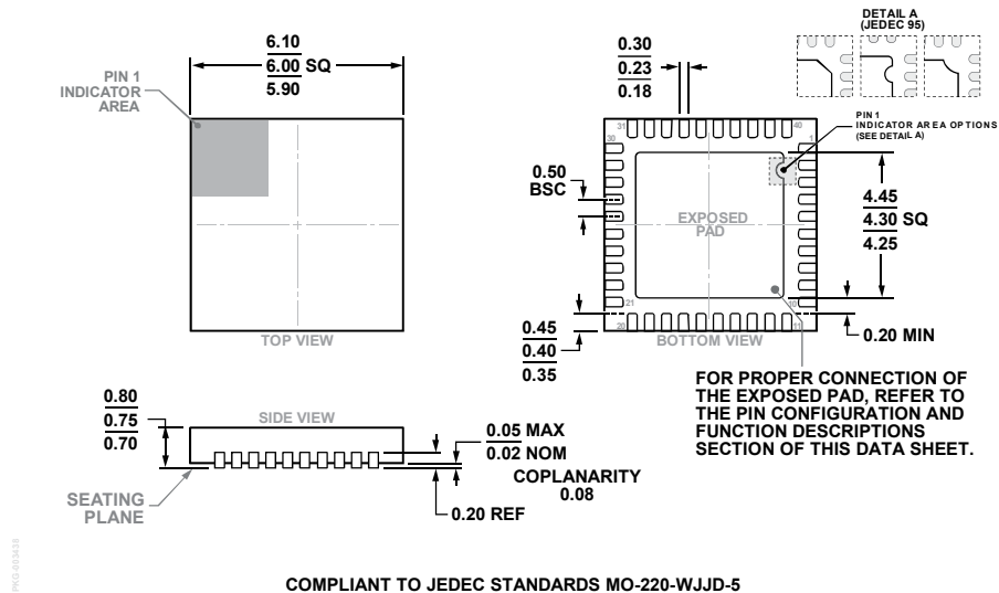
Figure 104. 40-Lead Lead Frame Chip Scale Package [LFCSP] 6 mm × 6 mm Body and 0.75 mm Package Height (CP-40-10) Dimensions shown in millimeters
