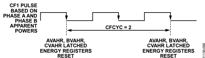
Figure 80. Synchronizing AVAHR and BVAHR with CF1
