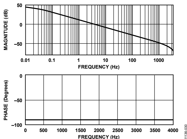
Figure 40. Combined Gain and Phase Response of the Digital Integrator
