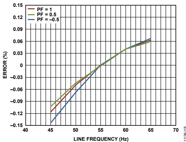
Figure 18. Fundamental Active Energy Error as a Percentage of Reading (Gain = +1) vs. Line Frequency over Power Factor over Frequency with Internal Reference and Integrator Off
