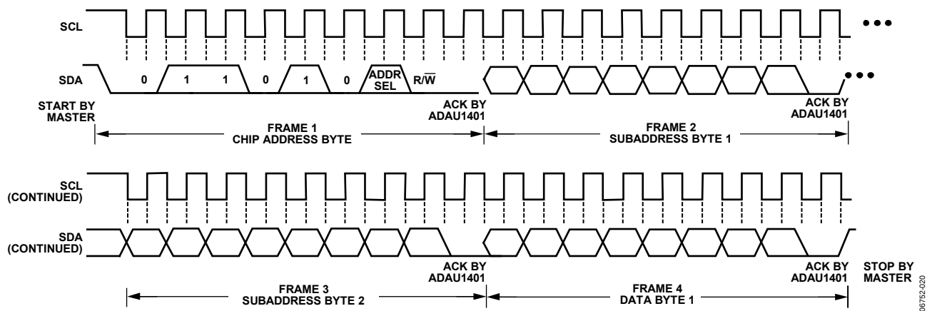
Figure 20. I 2 C Write to ADAU1401 Clocking
