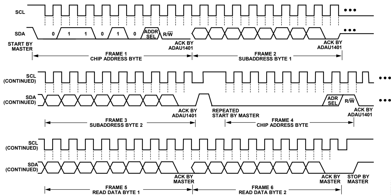
Figure 21. I 2 C Read from ADAU1401 Clocking
