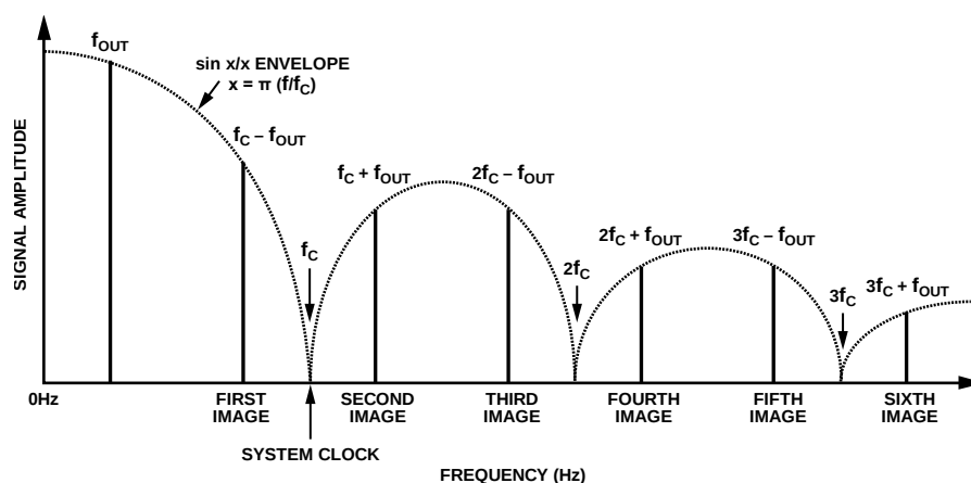
Figure 28. The DAC Output Spectrum
