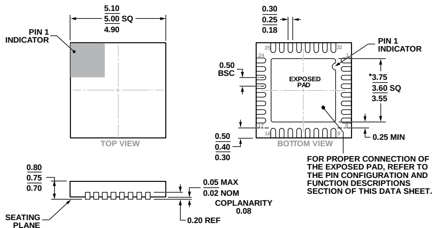
Figure 70. 32-Lead Lead Frame Chip Scale Package [LFCSP_WQ] 5 mm × 5 mm Body, Very Very Thin Quad (CP-32-12)
