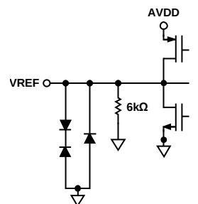
Figure 15. Equivalent VREF Circuit
