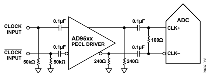
Figure 54. Differential PECL Sample Clock (Up to 625 MHz)
