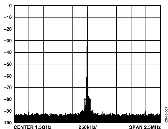
Figure 13. PLL Reference Spurs: VCO 1.5 GHz, f_{PFD} = 1 MHz
