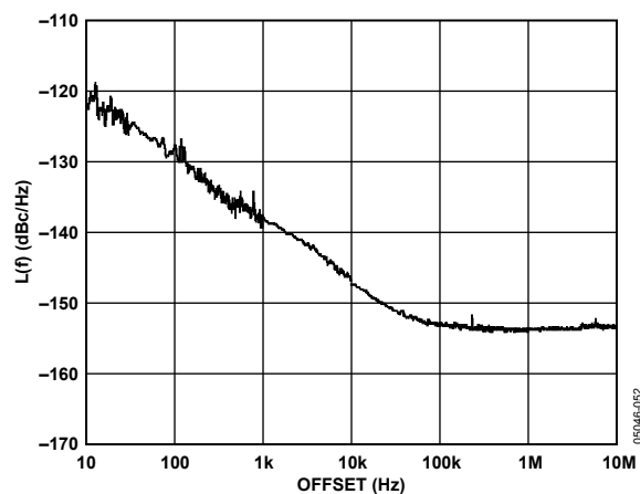
Figure 27. Additive Phase Noise—LVPECL DIV1, 622.08 MHz
