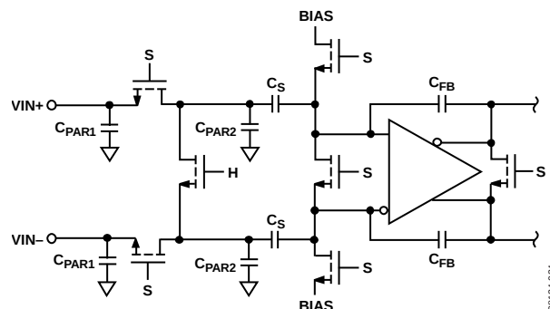
Figure 64. Switched-Capacitor Input
