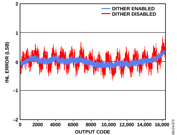
Figure 18. AD9258-80 INL with f_{IN} = 9.7 MHz
