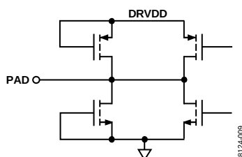
Figure 57. Digital Output
