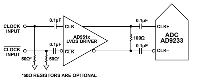
Figure 48. Differential LVDS Sample Clock
