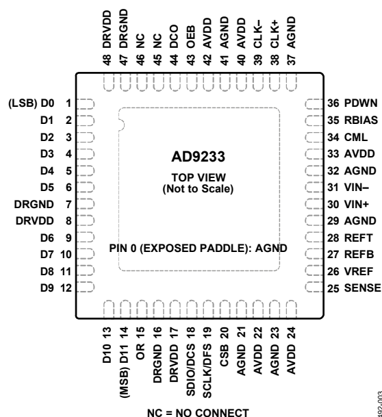
Figure 3. Pin Configuration
