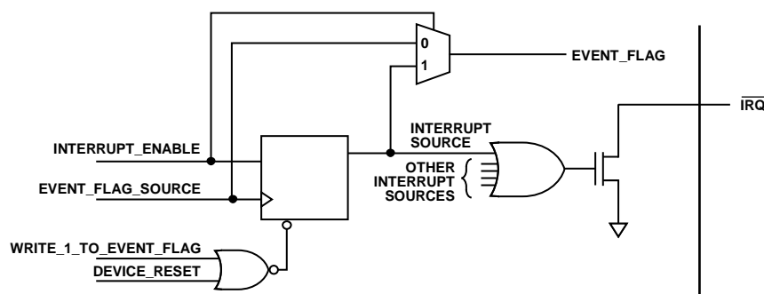
Figure 86. Simplified Schematic of \overline{IRQ} Circuitry
