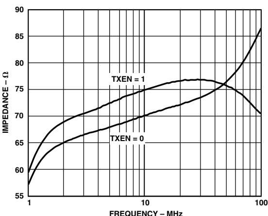
TPC 11. Output Impedance vs. Frequency
