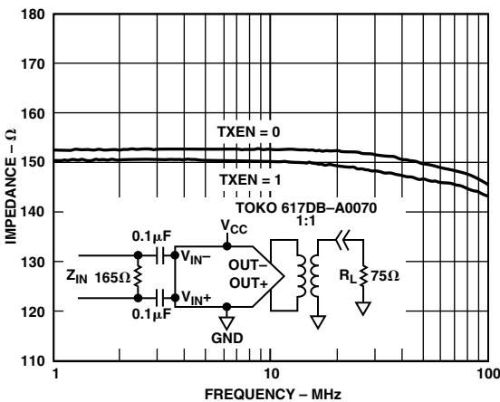
TPC 10. Input Impedance vs. Frequency
