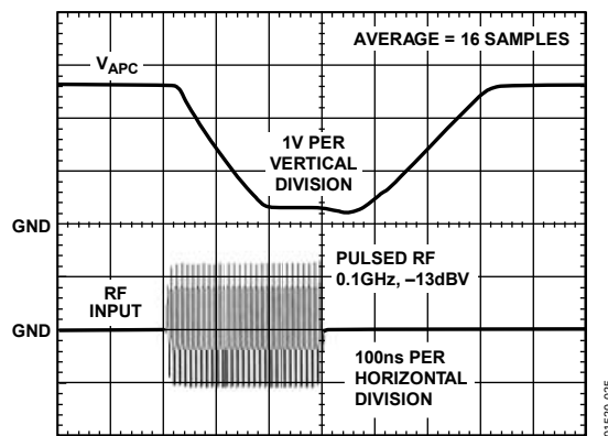
Figure 26. V_{APC} Response Time, Full-Scale Amplitude Change, Open-Loop
