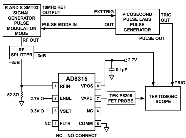
Figure 27. Test Setup for VAPC Response Time
