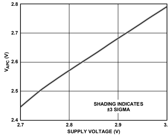
Figure 25. Maximum V_{APC} Voltage vs. Supply Voltage with 4 mA Load Current
