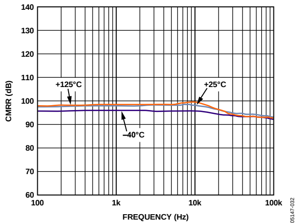
Figure 4. CMRR vs. Frequency and Temperature (Common-Mode Voltage < 5 V)
