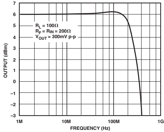
TPC 25. AD8048 Small Signal Frequency Response, G = +2
