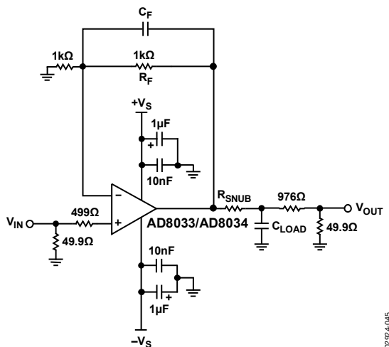
Figure 45. G = +2
