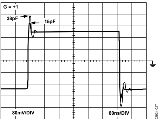
Figure 27. Small Signal Transient Response \pm 5\text{ V} (See Figure 44)
