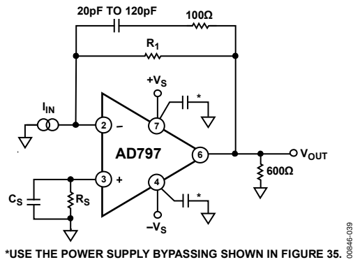
Figure 40. I-to-V Converter Connection
