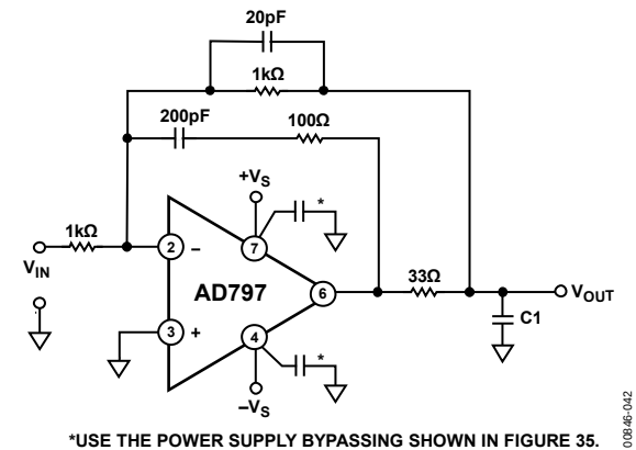
Figure 43. Recommended Circuit for Driving a High Capacitance Load
