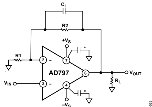
Figure 39. Low Noise Preamplifier
