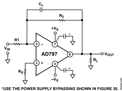
Figure 41. Inverting Amplifier Connection
