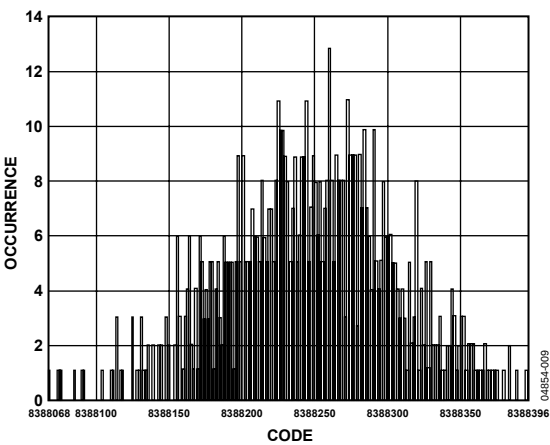
Figure 9. Noise Distribution Histogram for the AD7794 (Internal Reference, Gain = 64, Update Rate = 16.7 Hz, Chop Disabled, AMP-CM = 1)
