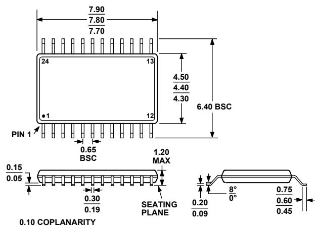
Figure 25. 24-Lead Thin Shrink Small Outline Package [TSSOP] (RU-24)
