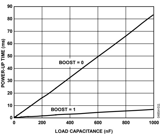
Figure 11. Bias Voltage Generator Power-Up Time vs. Load Capacitance
