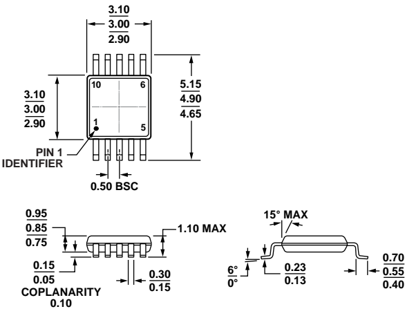
COMPLIANT TO JEDEC STANDARDS MO-187-BA Figure 17. 10-Lead Mini Small Outline Package [MSOP] (RM-10) Dimensions shown in millimeters
