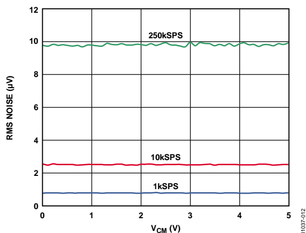
Figure 11. Noise vs. Common-Mode Input Voltage ( V_{REF} = 2.5\text{ V} )
