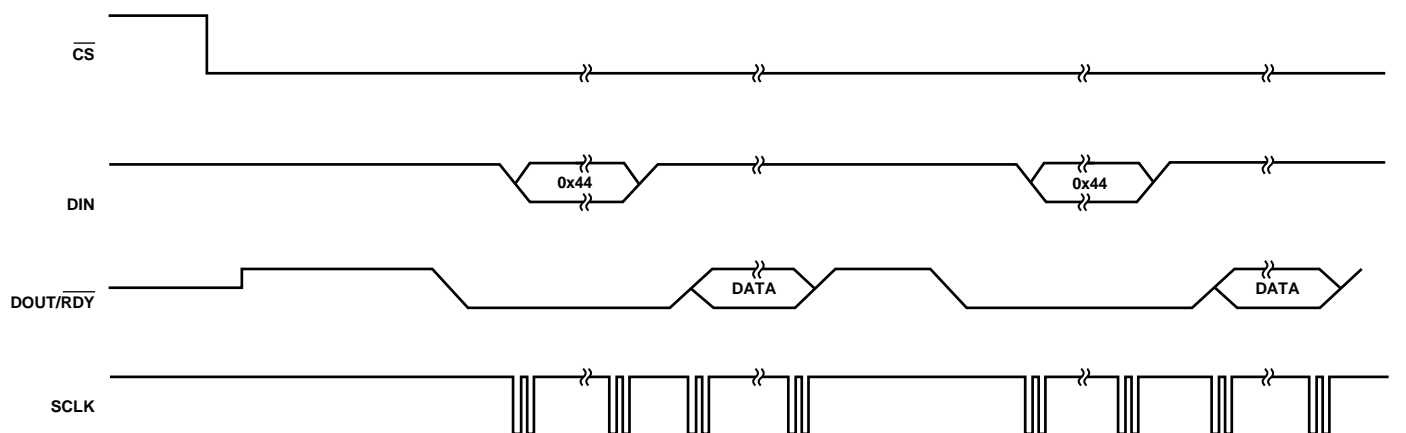
Figure 64. Continuous Conversion Mode
