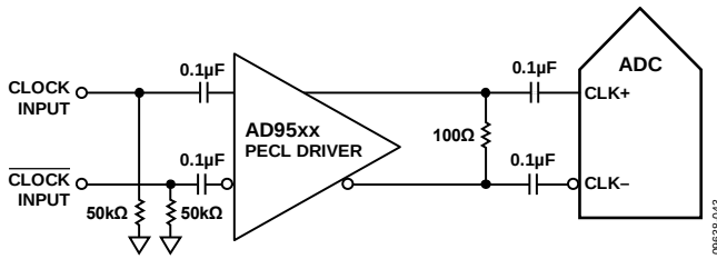
Figure 50. Differential LVDS Sample Clock (Up to 625 MHz)
