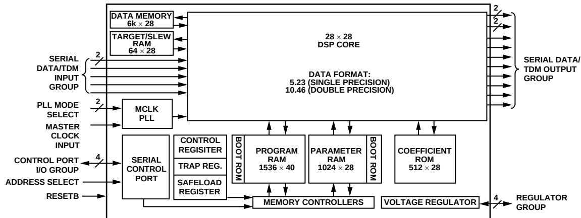
Figure 9. Block Diagram
