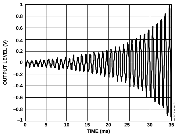
Figure 17. Slew RAM—Constant dB Update Increasing Ramp
