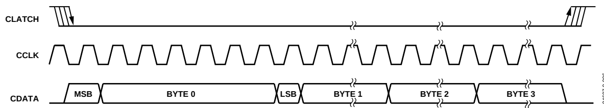
Figure 11. SPI Write Format (Single Write Mode)
