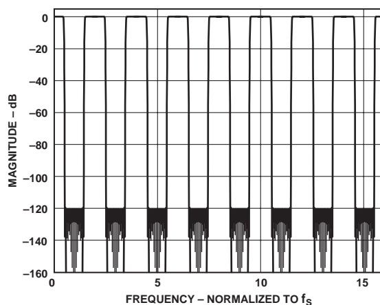
TPC 4. Second Half-Band Filter Response
