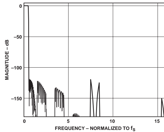
TPC 5. Composite Filter Response (AMC = 0)
