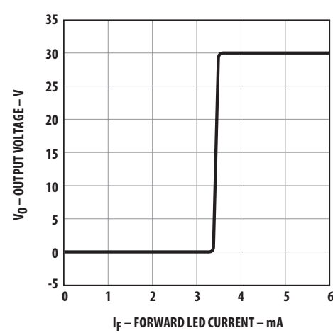
Figure 15 Transfer Characteristics
