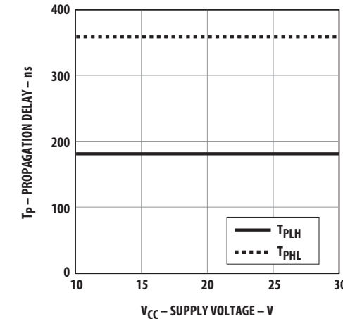
Figure 10 Propagation Delay vs. V_{CC}
