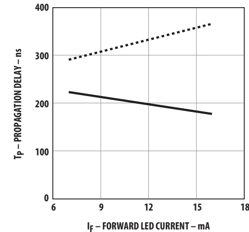
Figure 11 Propagation Delay vs. I_F
