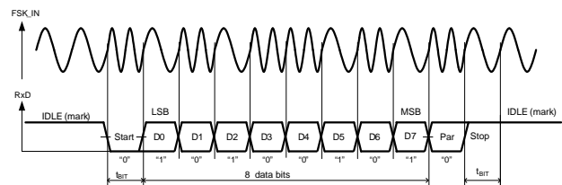
Figure 8. Modulation Timing
