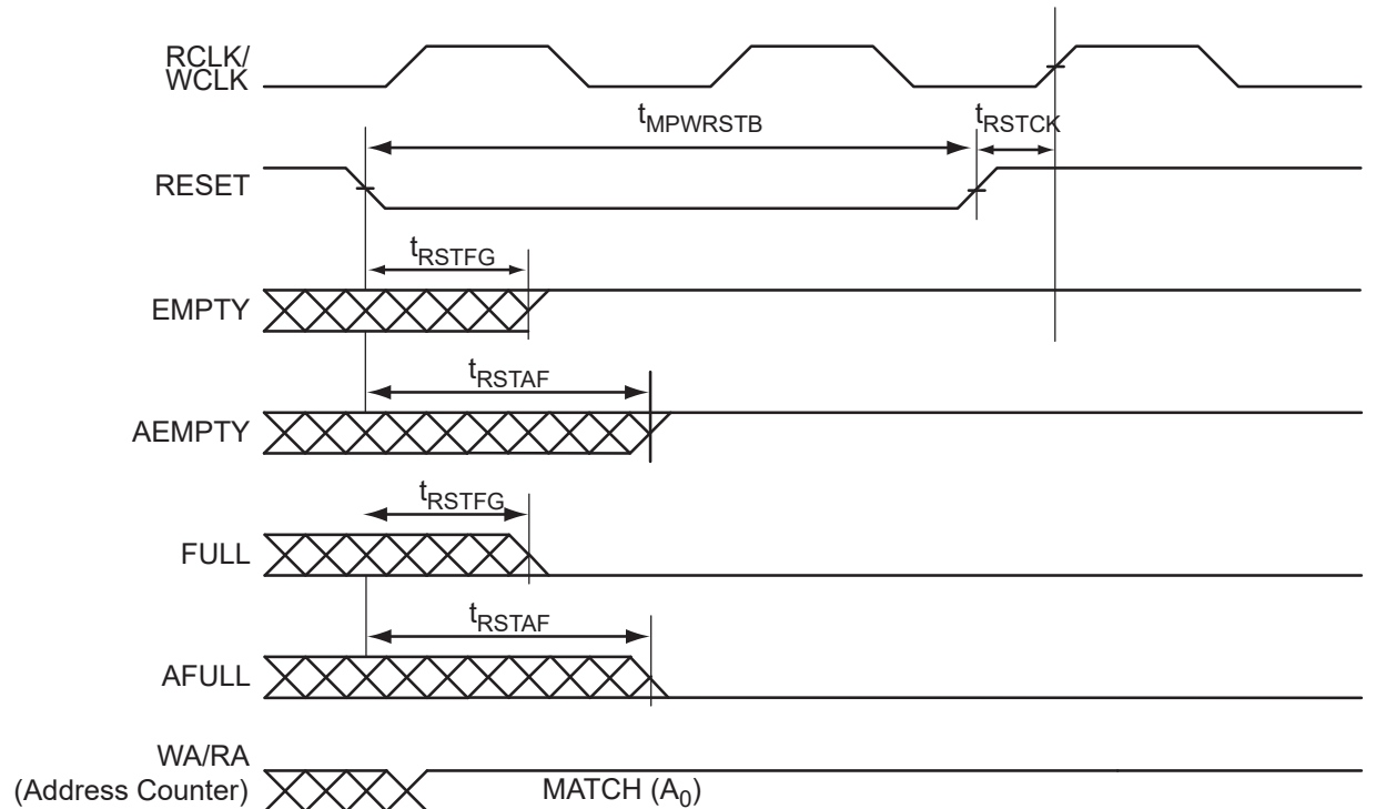
Figure 2-34 • FIFO Reset
