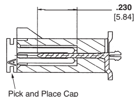
Section K-K
