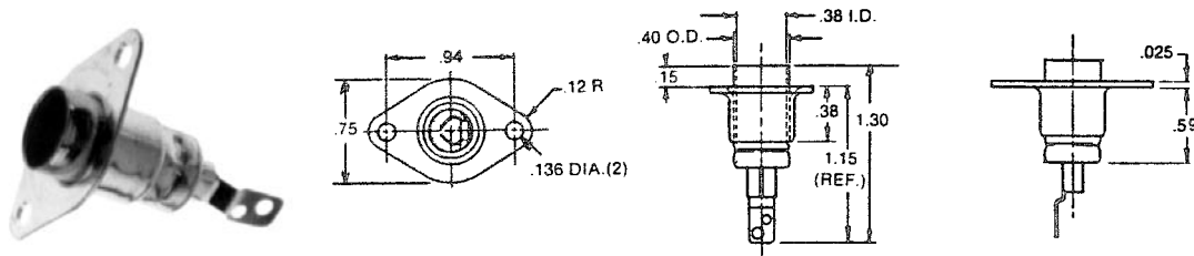
1207 Coaxial Antenna Jack
