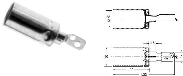
1235 Coaxial Antenna Jack
