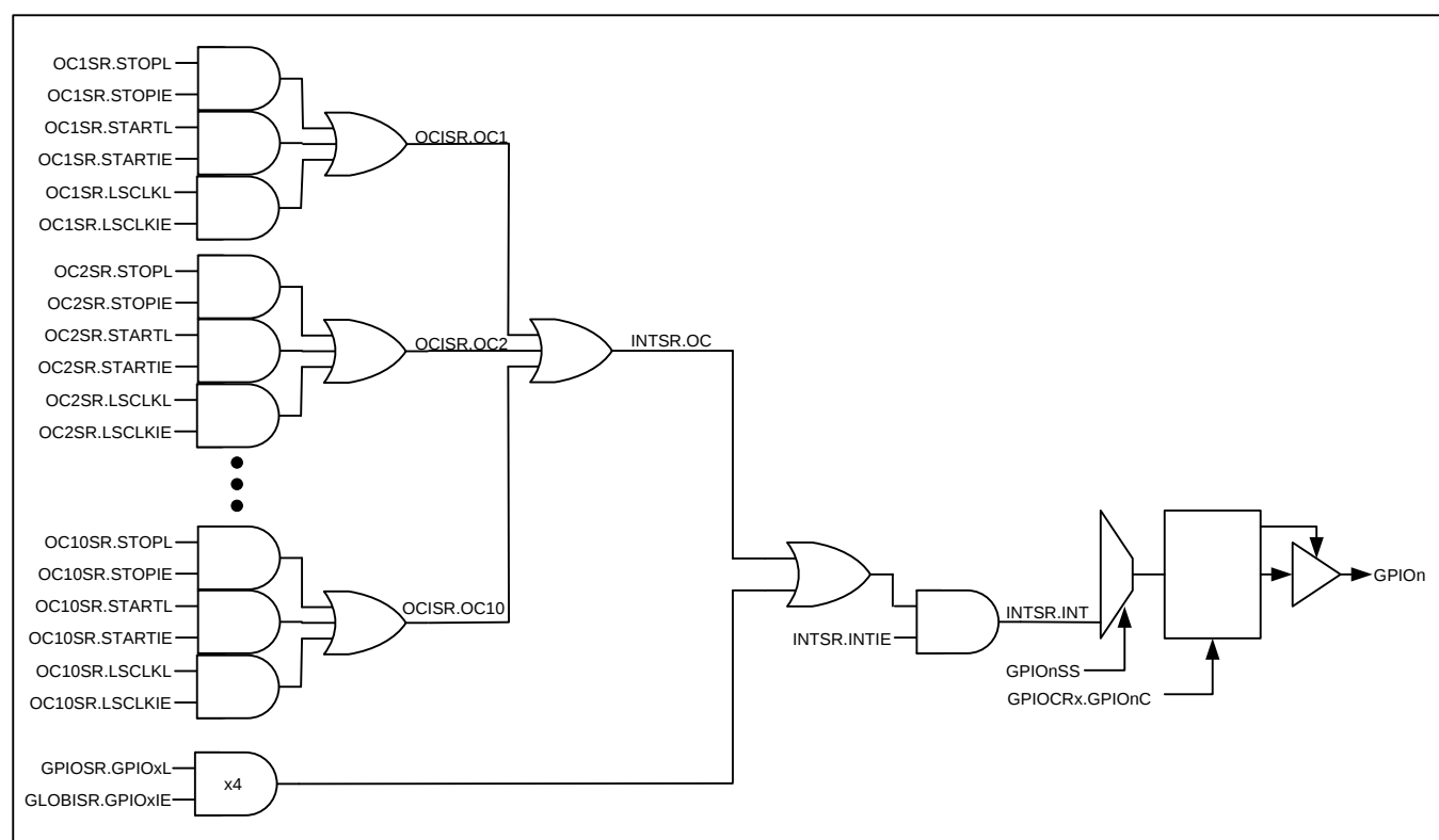
Figure 12 - Interrupt Structure
