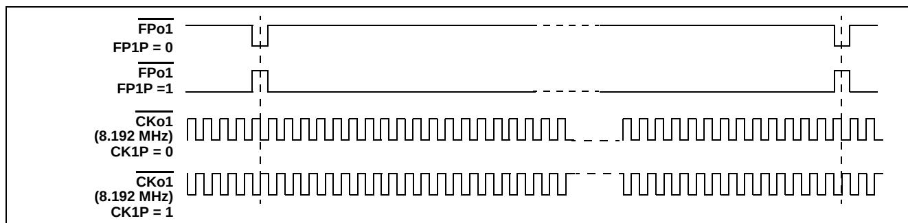
Figure 11 - FP1 and CK1 Output Timing when the CKFP1 Bit = 1
