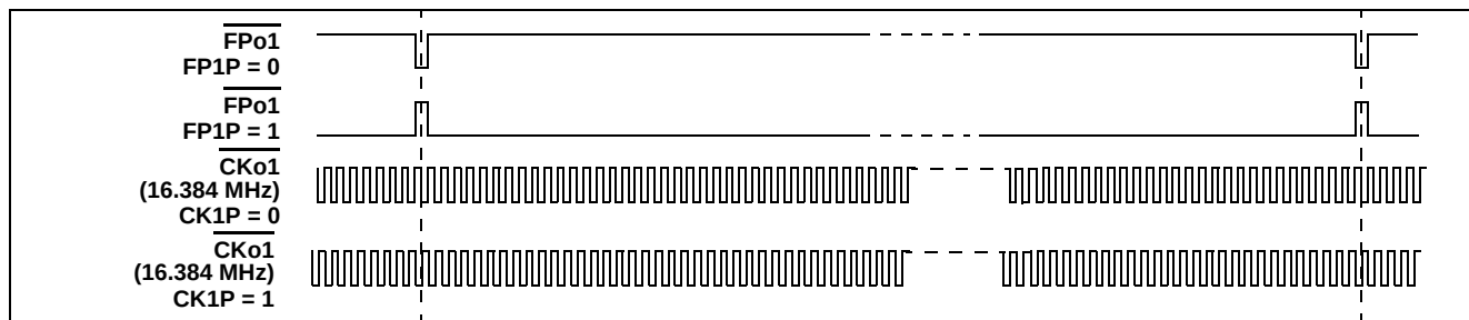
Figure 10 - FP1 and CK1 Output Timing when the CKFP1 Bit = 0
