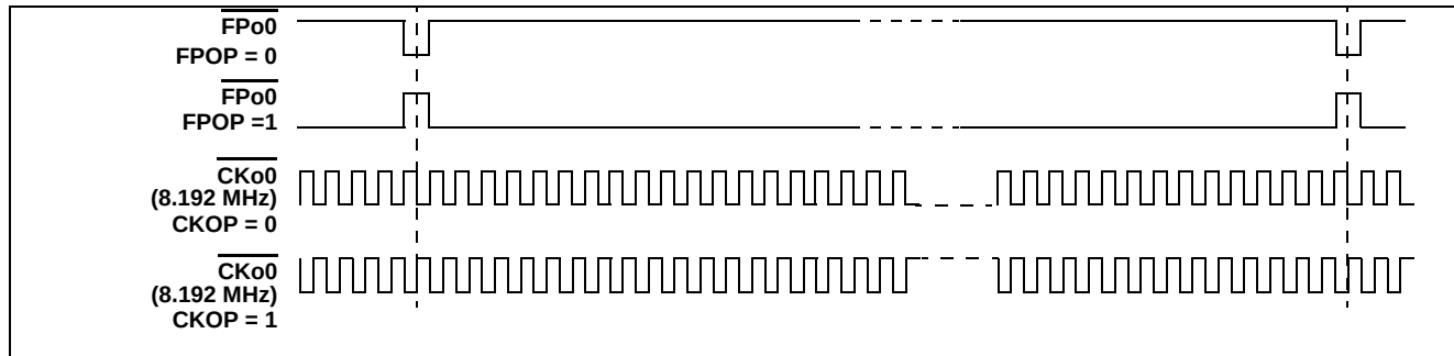
Figure 9 - FP0 and CK0 Output Timing when the CKFP0 Bit = 1
