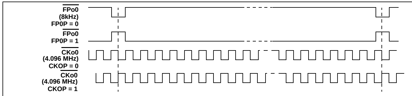
Figure 8 - FP0 and CK0 Output Timing when the CKFP0 Bit = 0
