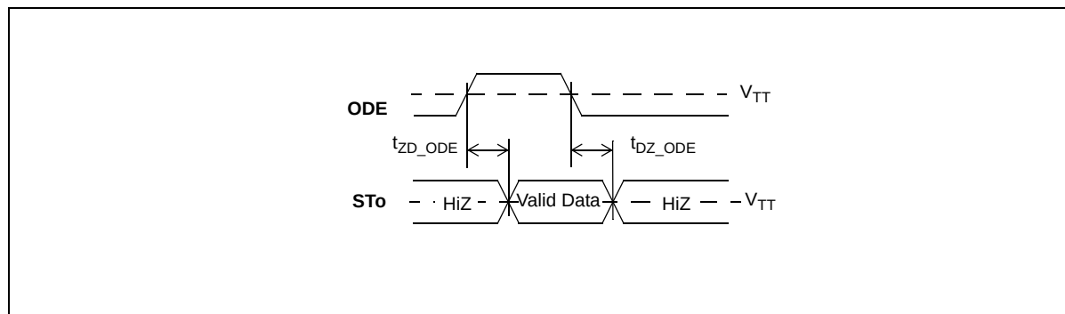
Figure 46 - Output Driver Enable (ODE)
