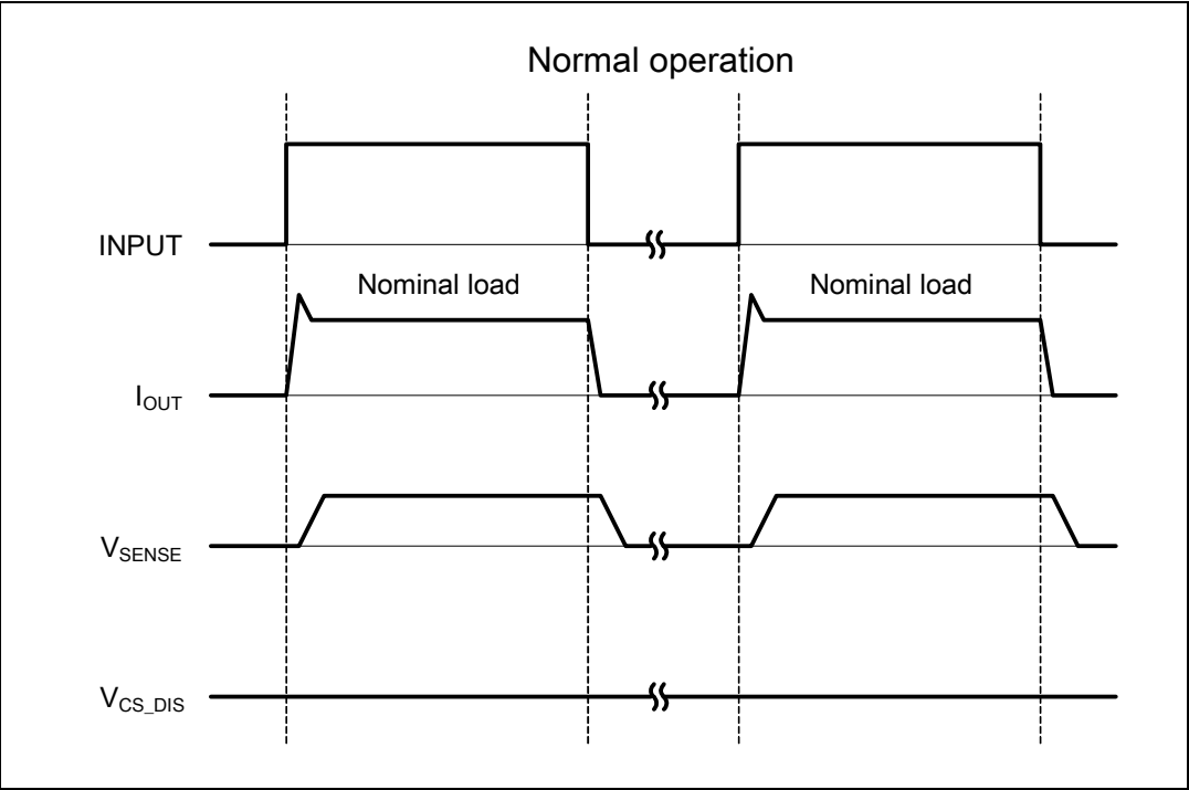
Figure 11. Normal operation
