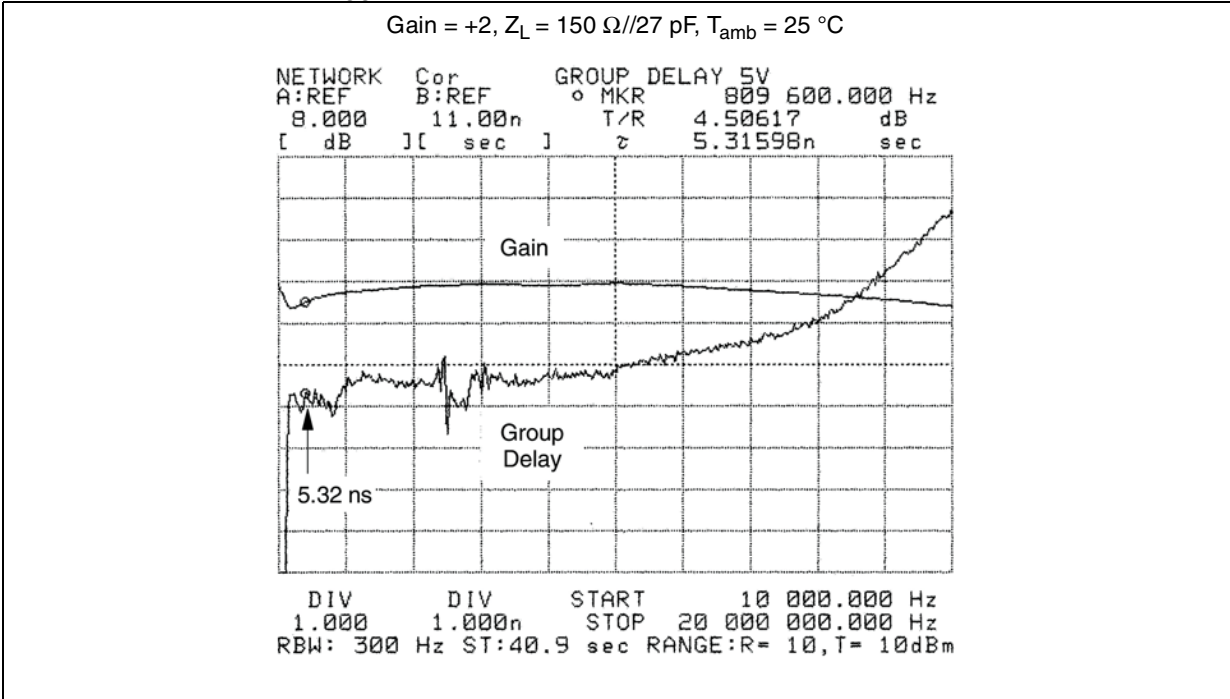
Figure 15. Group delay ( V_{CC} = \pm 2.5 V)
