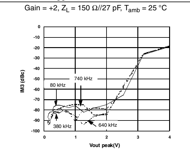
Figure 14. Third order intermodulation ( V_{CC} = \pm 2.5 V) (1)
