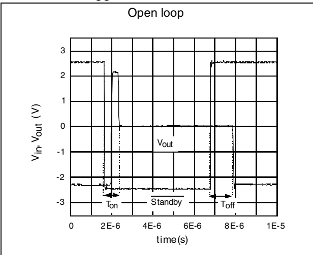
Figure 13. Standby mode - T_{on} , T_{off} ( V_{CC} = \pm 2.5 V)
