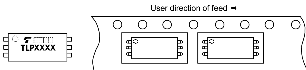
Orientation of Device in Relation to Direction of Tape Movement
