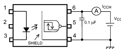
Fig. 13.1.4 ICCH Test Circuit
