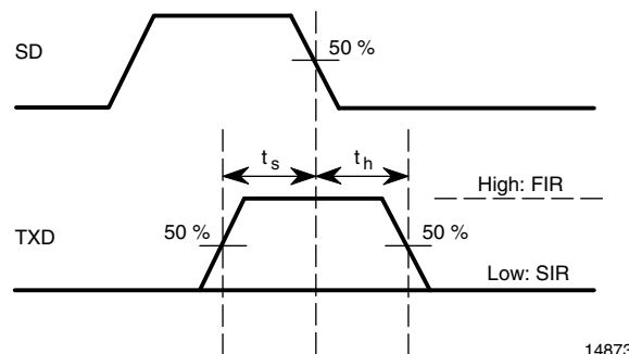
Fig. 4 - Mode Switching Timing Diagram
