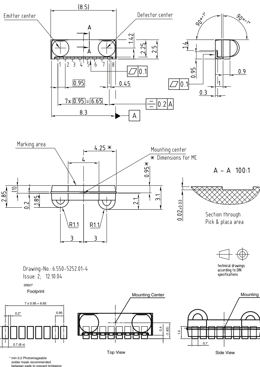
Fig. 8 - Package Drawing
