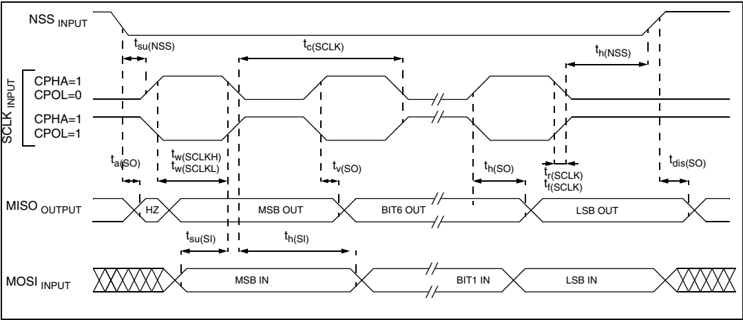
Figure 31. SPI slave timing diagram with CPHA = 1
