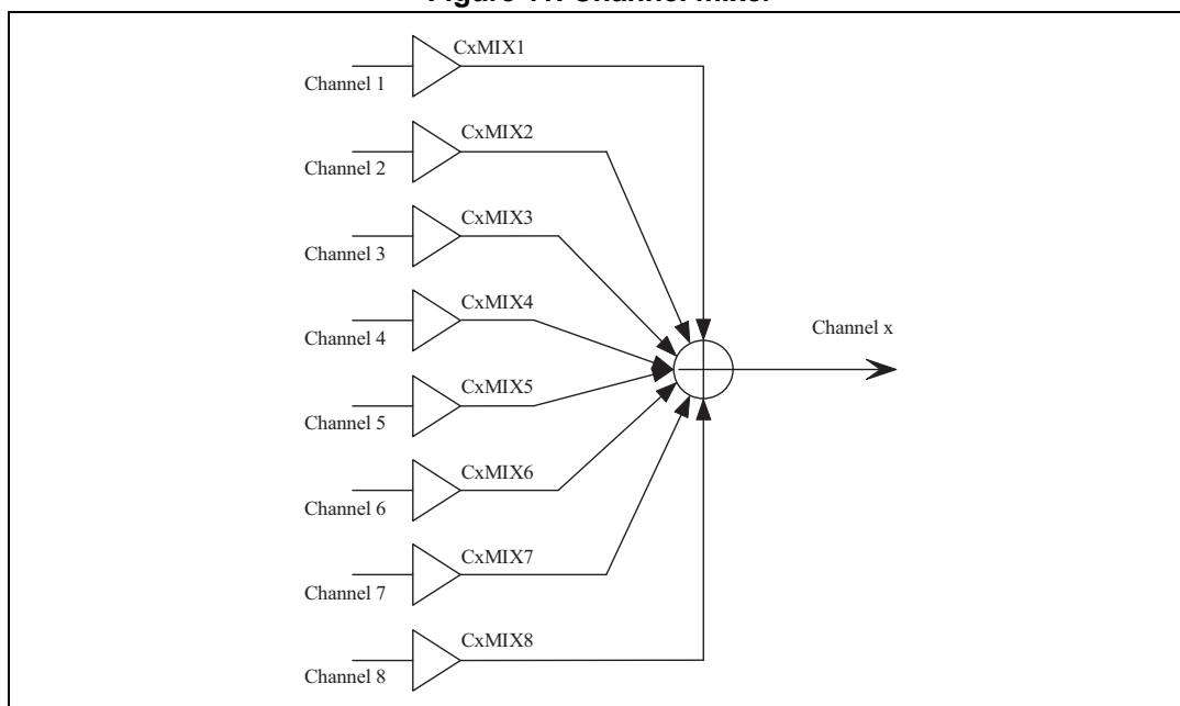
Figure 11. Channel mixer
