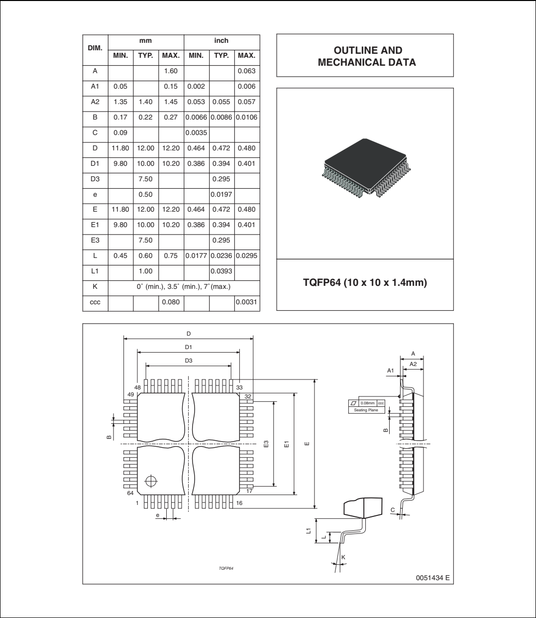
Figure 12. TQFP64 (10 x 10 mm) package dimensions
