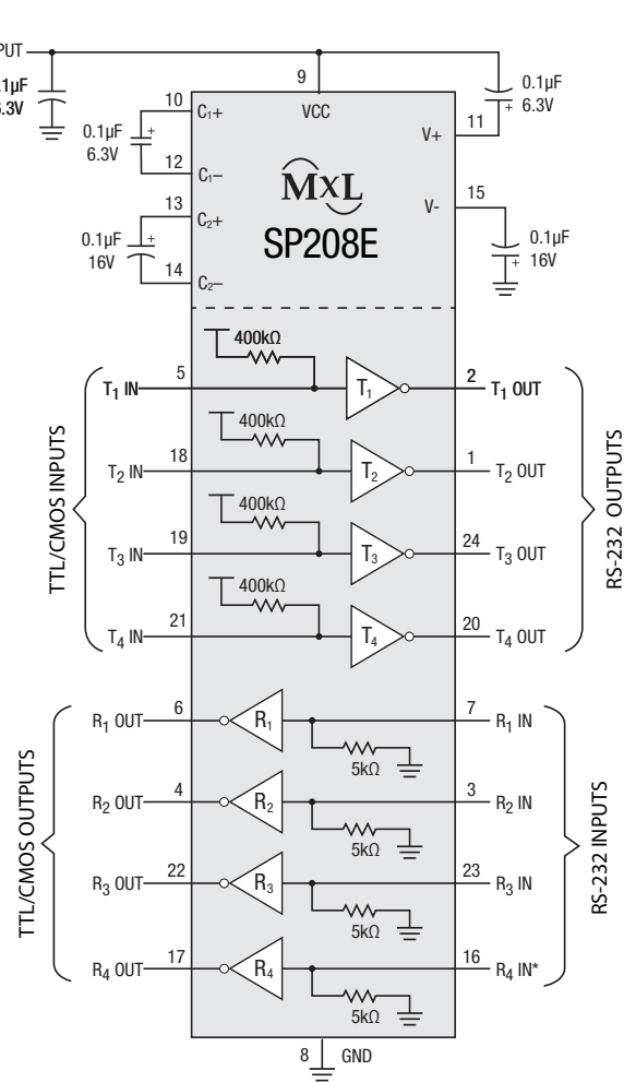
Figure 16: SP208E Typical Application
