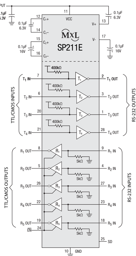
Figure 17: SP211E Typical Application
