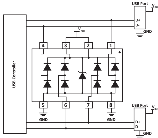
FIGURE 1 - DIFFERENTIAL MODE USB PROTECTION
