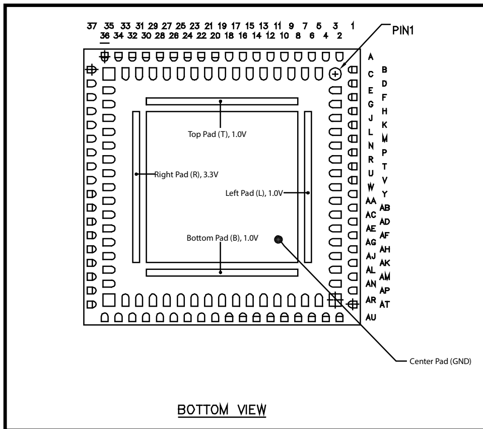
Figure 12-2 Package bottom view
