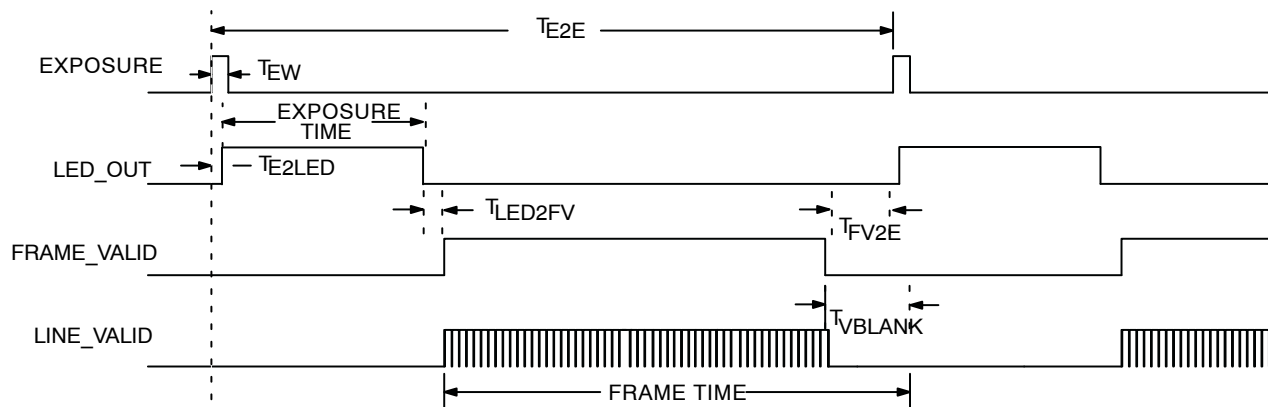
Figure 17. Snapshot Mode Frame Synchronization Waveforms
