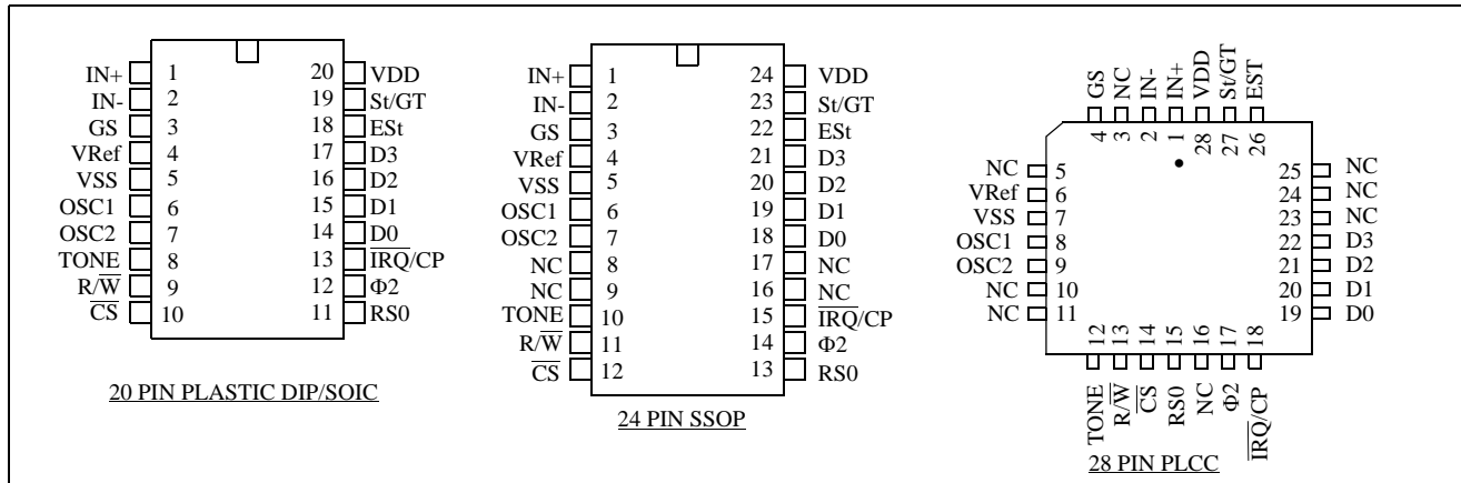
Figure 2 - Pin Connections
