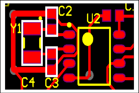
FIGURE 5-3: BOARD LAYOUT
