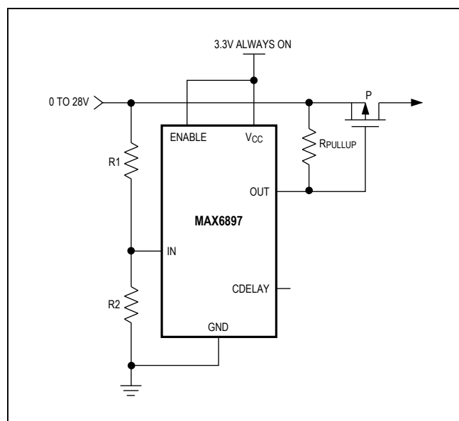
Figure 8. Overvoltage Protection
